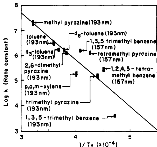
Figure 7. Logarithm of dissociation rate constant vs 1/T_V .
